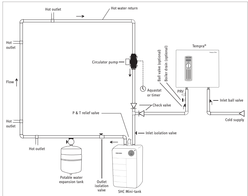
Tempra® and SHC Mini-Tank recirculation loop
