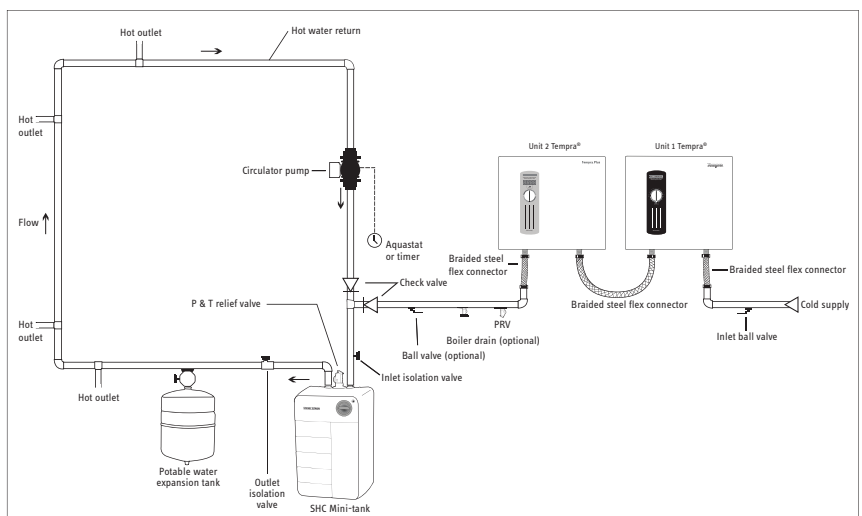
Tempra® and SHC Mini-Tank recirculation loop
