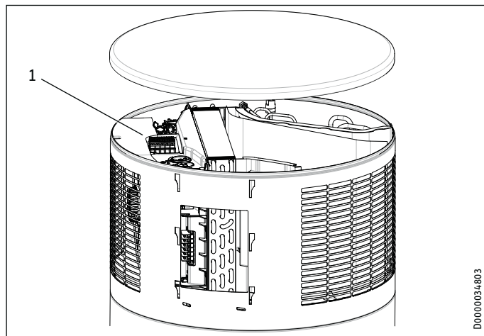
1 Terminal X0
