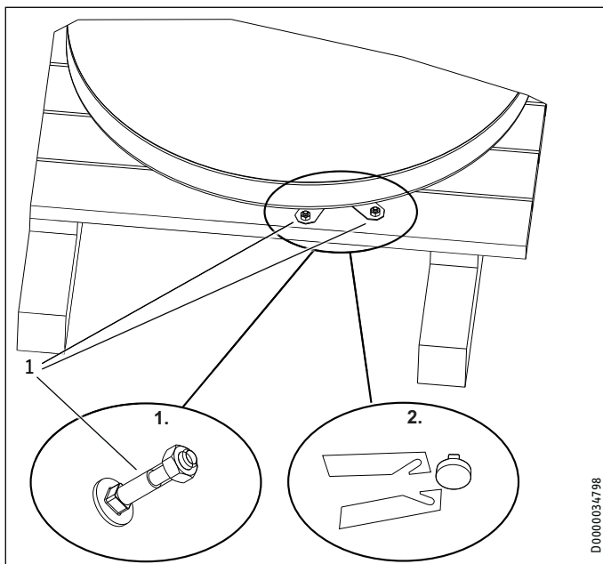
1 Metal bracket fixing bolt
