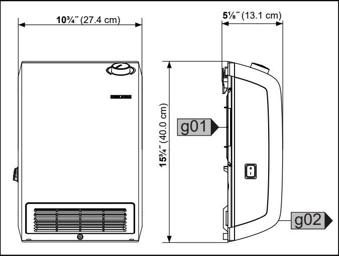
CK 150-1 Trend
